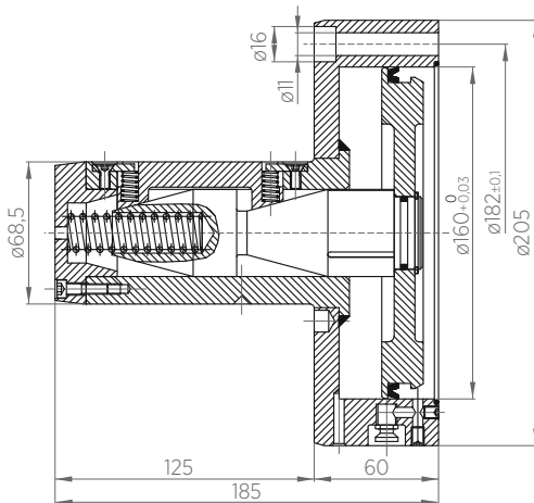
MX 16.3 chuck
