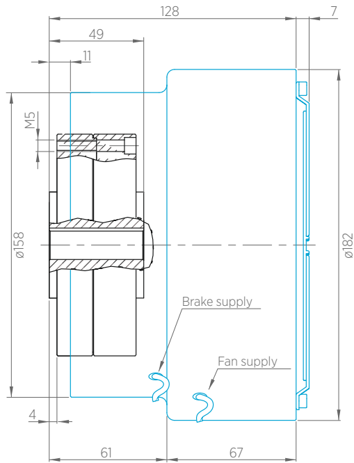
B.121.V with fan
