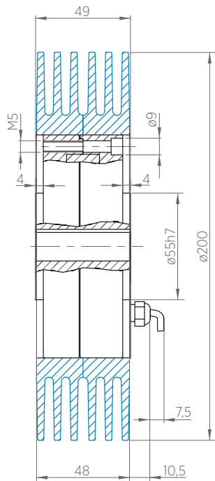
B.121.R with radiator
