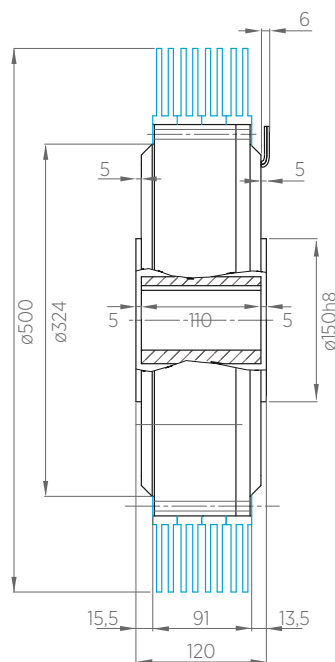
B.5000.R with radiator
