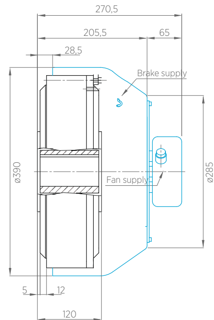
B.5000.V with fan
